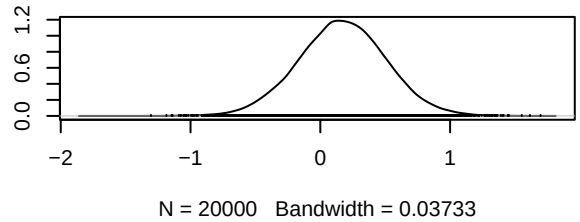
Density of d.I.II
